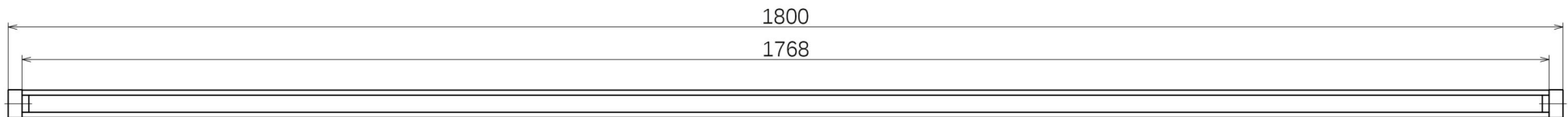
Notch Cutting Dimension
